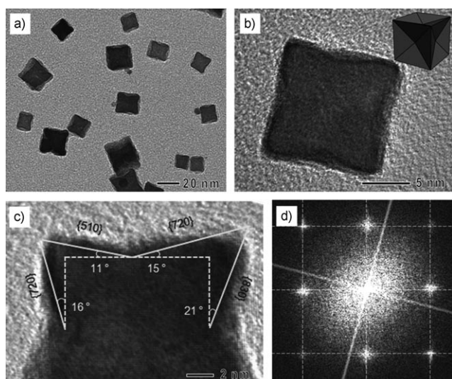
Figure 1. a) TEM and b, c) HRTEM images of Pt concave nanocubes synthesized by continuously adding an aqueous \text{NaBH}_4 solution and a mixture of \text{K}_2\text{PtCl}_4 , \text{KBr} , and \text{Na}_2\text{H}_2\text{P}_2\text{O}_7 using two syringe pumps into deionized water held at 95^\circ\text{C} . The injection rate was 67\ \mu\text{L}\cdot\text{min}^{-1} , and the \text{KBr}/\text{Na}_2\text{H}_2\text{P}_2\text{O}_7 ratio was 3:1. d) FT pattern of the concave nanocube shown in (c) recorded along the [001] zone axis.
